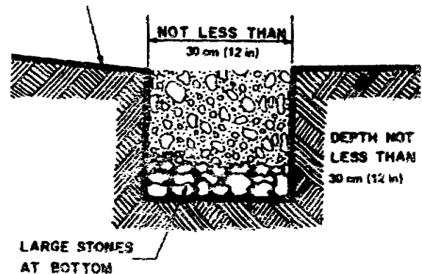
Figure 1-36. Sump for shelter drainage.
